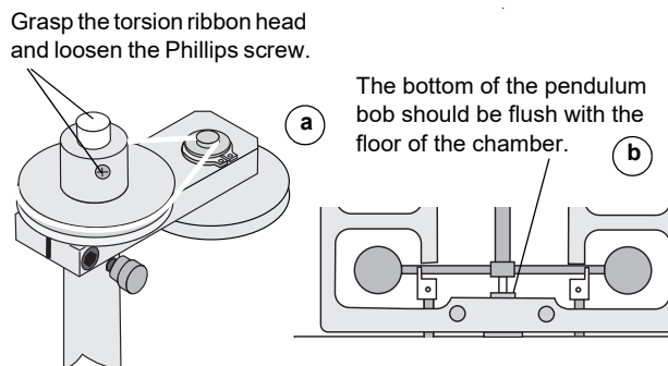
Figure 6: Adjusting the height of the pendulum bob
